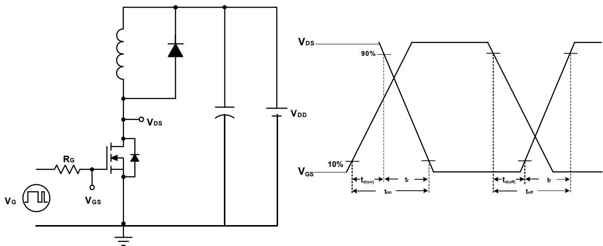
Figure 14. Unclamped Inductive Switching Test Circuit and Waveforms
